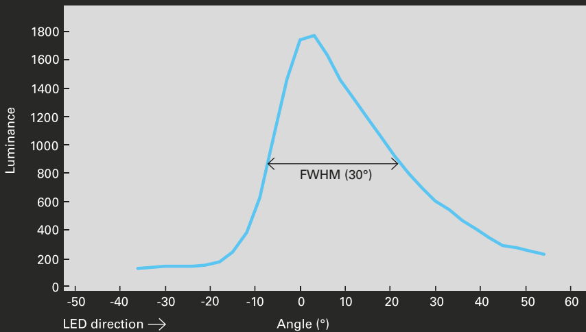
Angular luminance distribution
